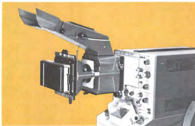
Corrector lens in place. Adapter frame secured to Type 576 accepts C-12 or C-27 with standard 5-inch round CRT adapter.
